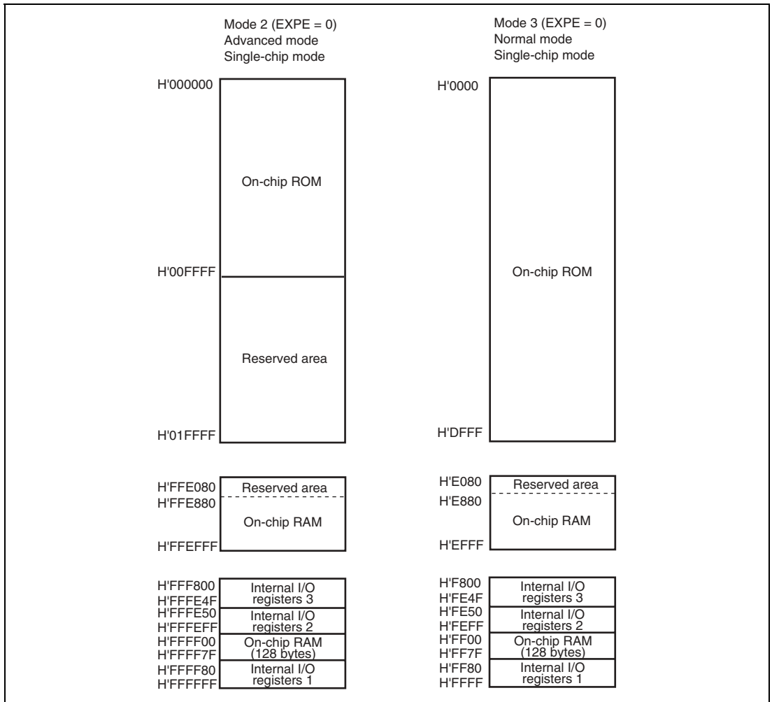
Figure 3.1 Address Map for H8S/2111B-B
